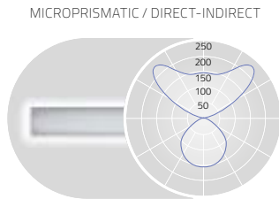
UGR \leq 19 for Medium Power (X=4H, Y=8H, S=0.25H) DIRECT: ca. 45% INDIRECT ca. 55%
