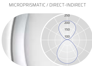
UGR \leq 16 (X=4H, Y=8H, S=0.25H) DIRECT: ca.50% INDIRECT ca.50%
