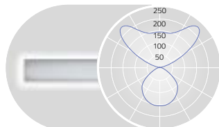
MICROPRISMATIC / DIRECT-INDIRECT
