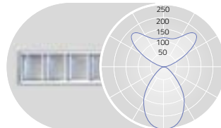
UGR \leq 16 (X=4H, Y=8H, S=0.25H) DIRECT: ca.40% INDIRECT ca.60%
