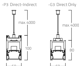
MICROPRISMATIC / DIRECT-INDIRECT
