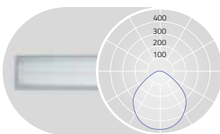
UGR<math>\leq 19</math> for Low Power (X=4H, Y=8H, S=0.25H) DIRECT 100%
