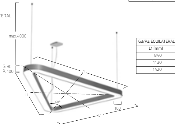
MICROPRISMATIC / DIRECT-INDIRECT
