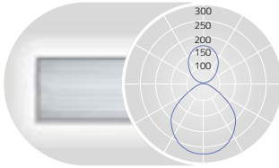
UGR<sub>s19</sub> for Low Power (X=4H, Y=8H, S=0.25H) DIRECT: ca. 60% INDIRECT ca. 40%
