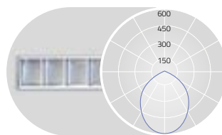
UGR<math>\leq 19</math> for Medium Power (X=4H, Y=8H, S=0.25H) DIRECT 100%
