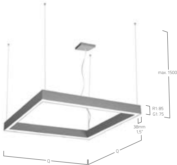
MICROPRISMATIC / DIRECT-INDIRECT
