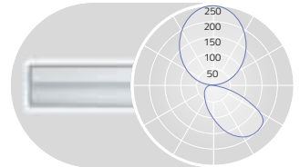
WALLWASHER | DIRECT-INDIRECT
