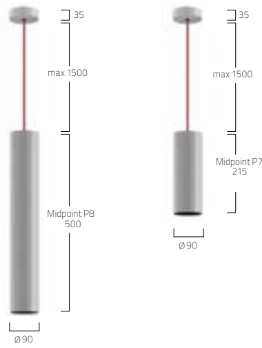
SPOT 10° LED ENGINE ECO, MEDIUM POWER
