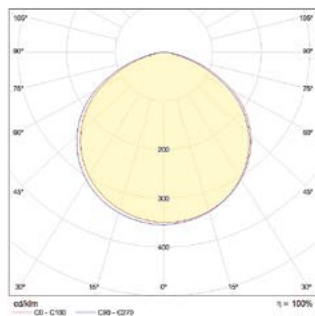
LVK PFLH150-120D
