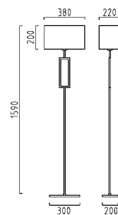
1 x E27, max. 60 W 17/1138.10/9243
