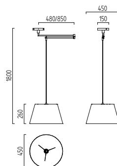
Schirm Chintz anthrazit / shade chintz anthracite 16/1847.04/9283
