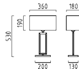
1 x E27, max. 60 W 19/1139.10/9245
