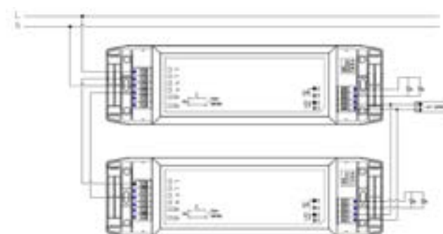
1-10 V Dim
